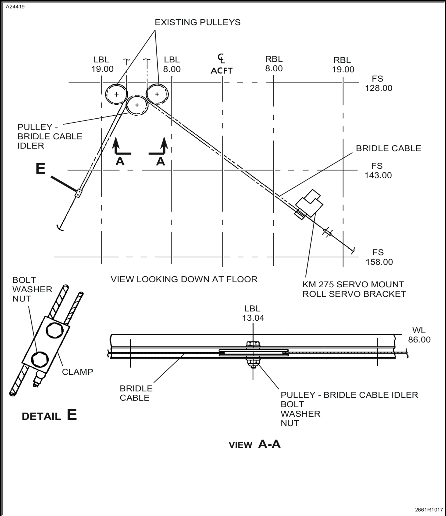
Figure 503 : Sheet 4 : Aileron Rigging (Airplanes with KAP-150 Autopilot and KFC-150, KFC-225 Flight Control System Installed)
