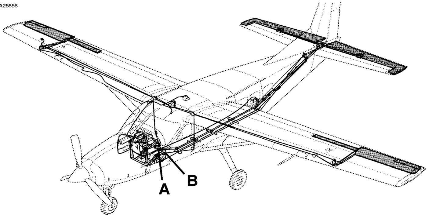
Figure 501 : Sheet 1 : Aileron Rigging (Airplanes with 400B and 400B IFCS Autopilots Types AF-550A and IF-550A Installed)
