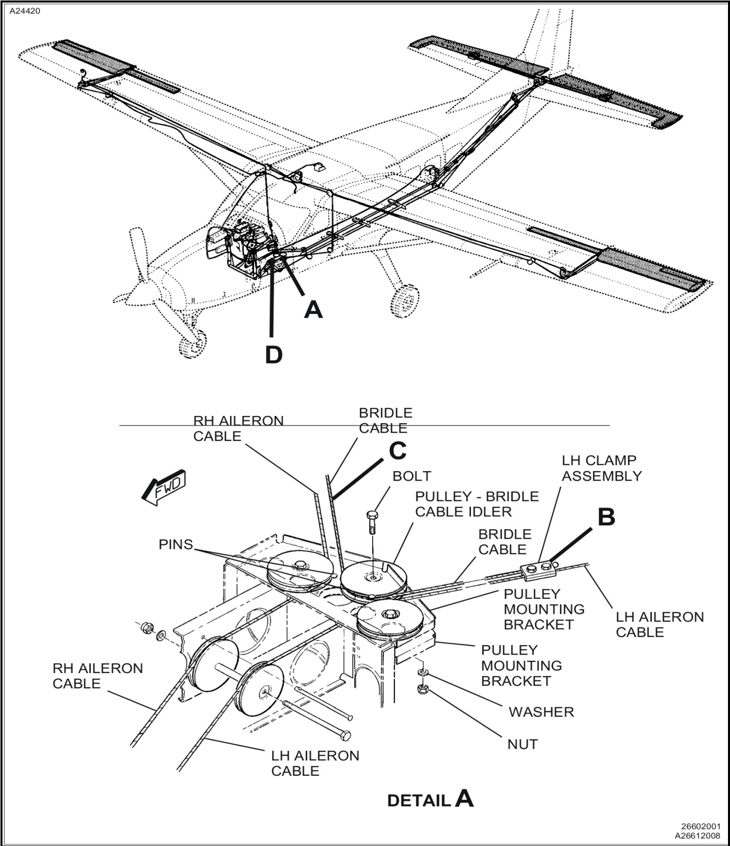
Figure 503 : Sheet 1 : Aileron Rigging (Airplanes with KAP-150 Autopilot and KFC-150, KFC-225 Flight Control System Installed)
