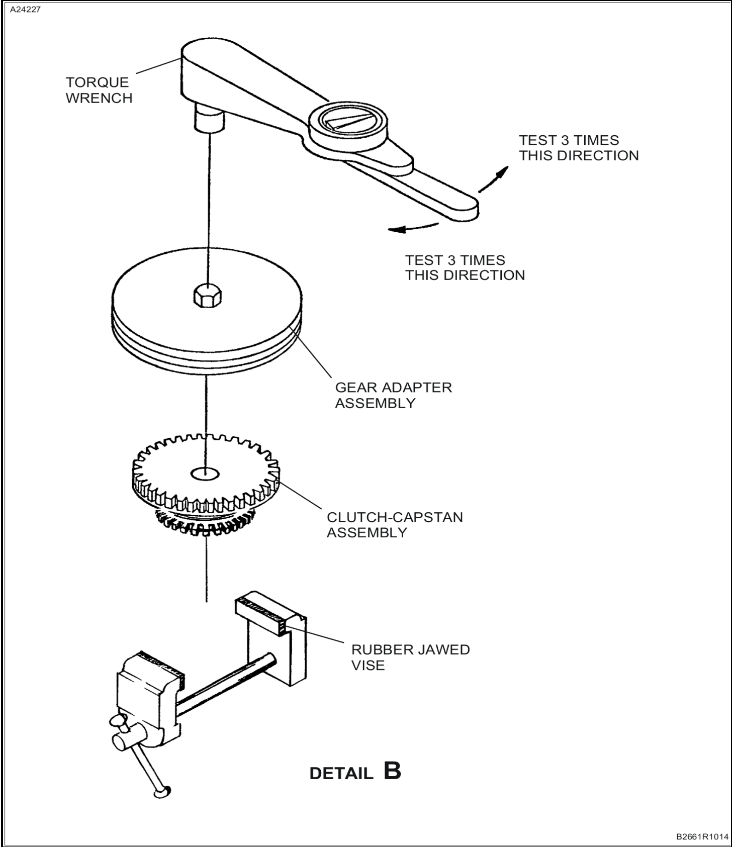
Figure 502 : Sheet 3 : Clutch Adjustment
